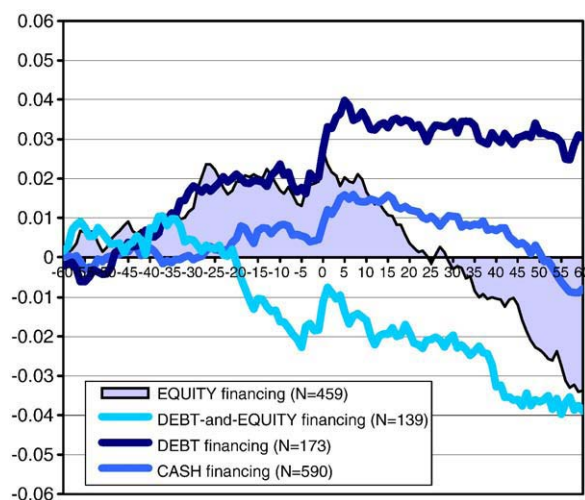
Fig. 3. Figure 3 shows the daily evolution of the cumulative average abnormal returns (CAARs) for different subsamples of bidding firms starting 60 trading days before the bid announcement up to 60 days after the bid. The subsamples are classified by the sources of financing. The number of observations in each subsample is reported in brackets. The day of the bid announcement is denoted as day 0. Abnormal returns are computed as the difference between the realized and market model benchmark returns. For each firm we calculate daily benchmark returns using MSCI-Europe index returns and the market model parameters are estimated over 240 days starting 300 days prior to the acquisition announcement.
