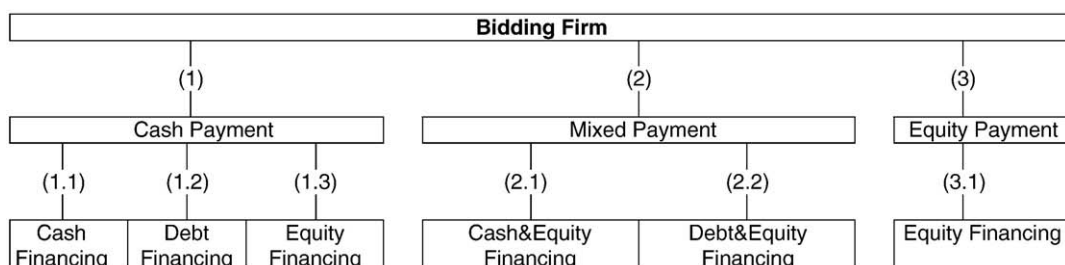
Fig. 1. Specification of the payment-financing nested logit model.
