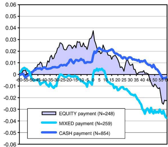
Fig. 2. Note: Figure 2 shows the daily evolution of the cumulative average abnormal returns (CAARs) for different subsamples of bidding firms starting 60 trading days before the bid announcement up to 60 days after the bid. The subsamples are classified by the means of payment. The number of observations in each subsample is reported in brackets. The day of the bid announcement is denoted as day 0. Abnormal returns are computed as the difference between the realized and market model benchmark returns. For each firm we calculate daily benchmark returns using MSCI-Europe index returns and the market model parameters are estimated over 240 days starting 300 days prior to the acquisition announcement.
